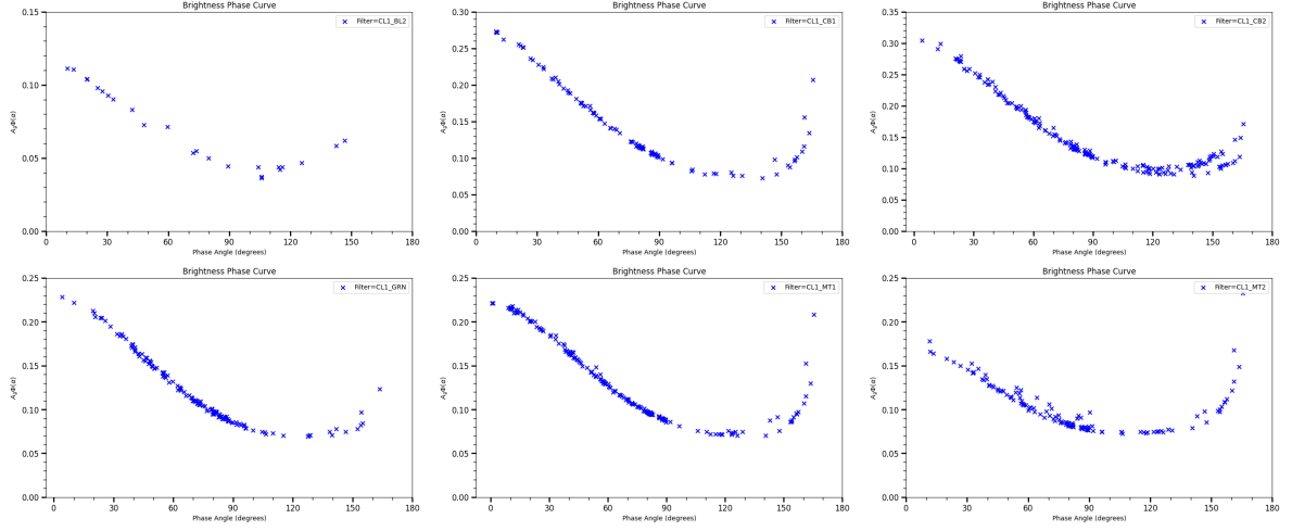
Figure 1: Brightness phase curves of Titan from 0 to 180 degrees phase angle for different filters. Brightness decreases from 0 to 90 degrees and plateaus between 90 and 130 degrees, especially in the MT2 filter ( 0.7254 \mu\text{m} ). Brightness increases again from 130 to 170 degrees, with the MT1 filter ( 0.6171 \mu\text{m} ) showing higher brightness at larger phase angles due to Titan's atmosphere and sunlight scattering.
